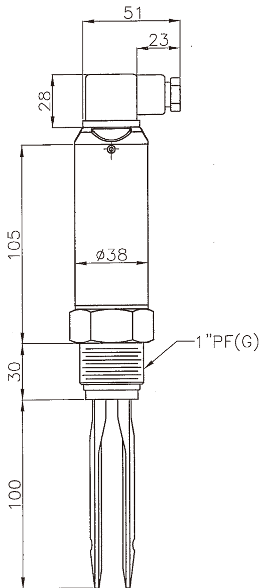
VIBRATING PROBE LEVEL SWITCH
